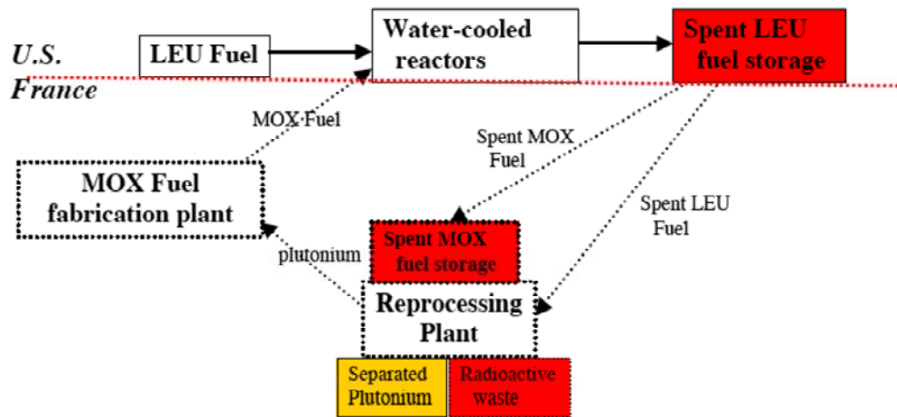
Figure 1. Currently competing spent fuel management strategies. Above the dotted horizontal line, the “once-through” fuel cycle as currently practiced in the U.S. and many other countries. Low-enriched uranium (LEU) fuel is irradiated in a light-water reactor and then stored. The reprocessing and recycle system that is in operation in France and soon will be in Japan is shown below the line. It involves the separation and recycle of the plutonium in “mixed-oxide” (MOX, uranium-plutonium) fuel. The spent MOX fuel is then stored. Because of the high cost of reprocessing, the cost of this MOX fuel is much higher than the cost of LEU fuel and most countries have decided that it is not worthwhile.
